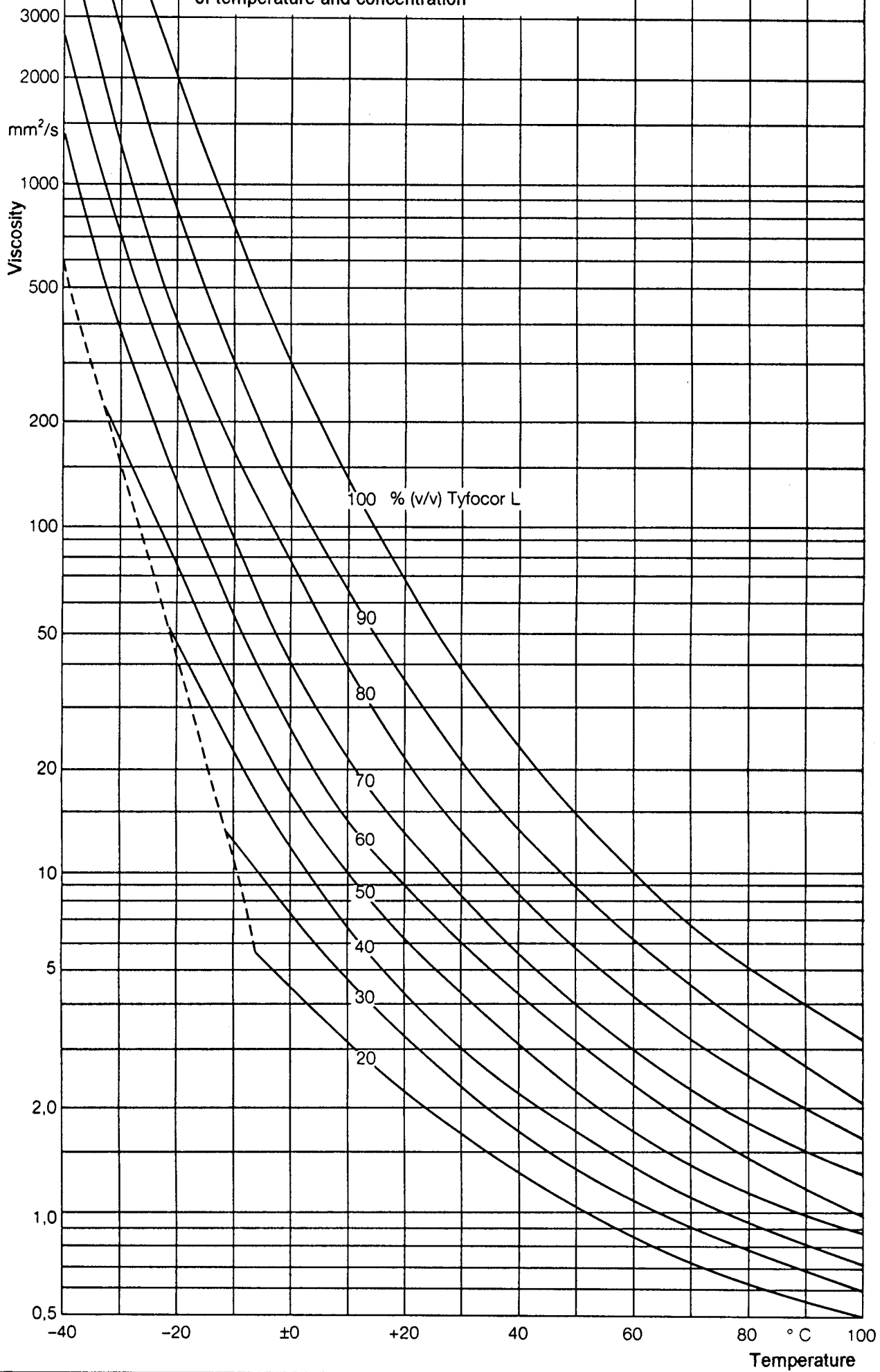
Viscosity of aqueous Tyfocor L mixtures as a function of temperature and concentration
