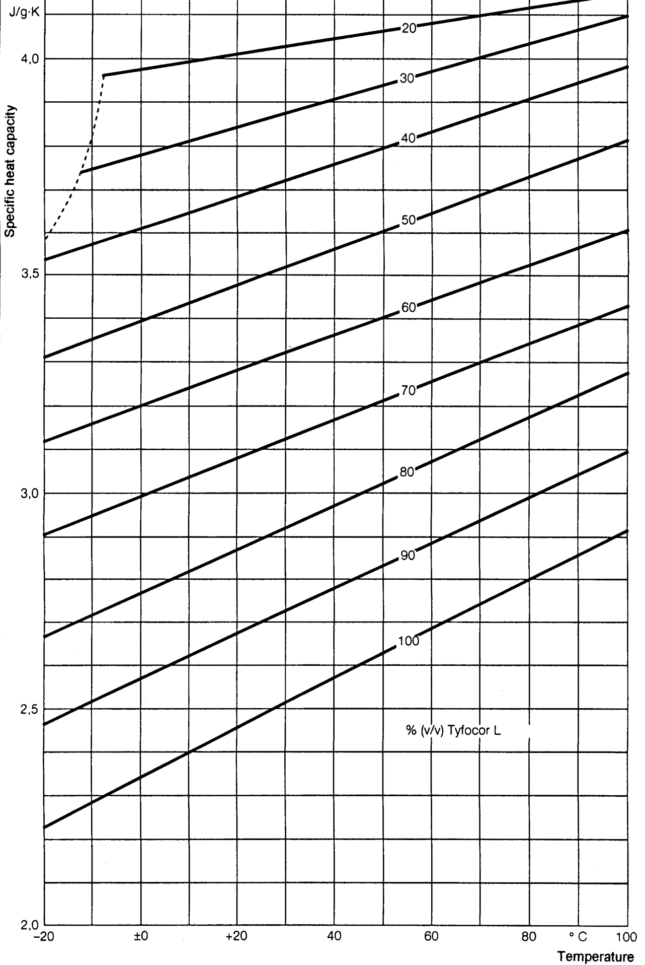
Specific heat capacity of aqueous Tyfocor L mixtures as a function of temperature and concentration
